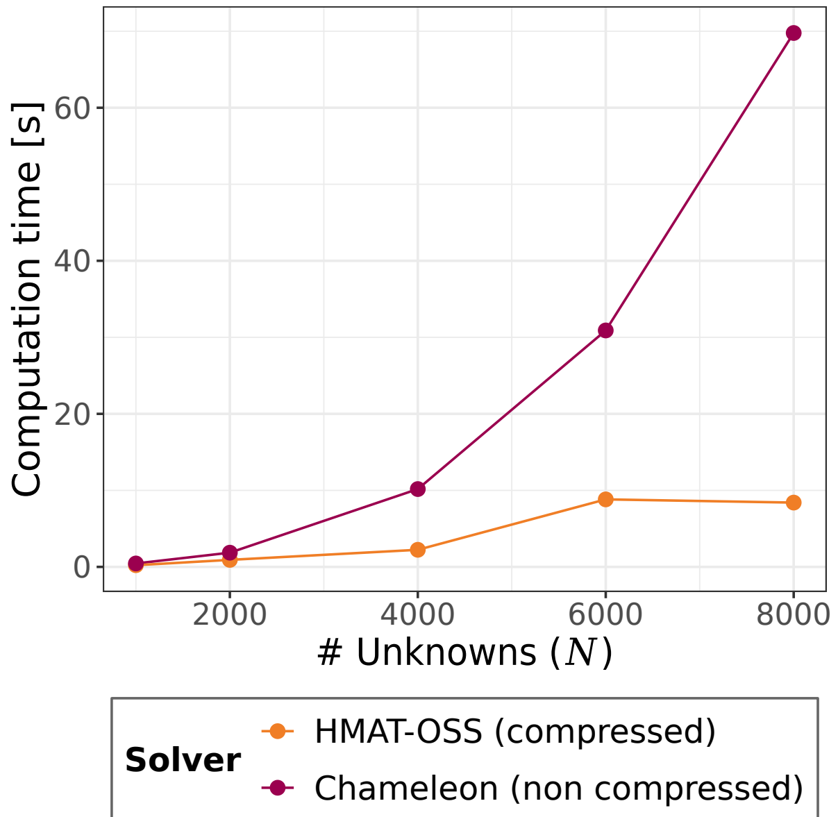
FIGURE 2: Computation times of sequential runs of HMAT-OSS and Chameleon on coupled sparse/dense FEM/BEM linear systems of varying size.
