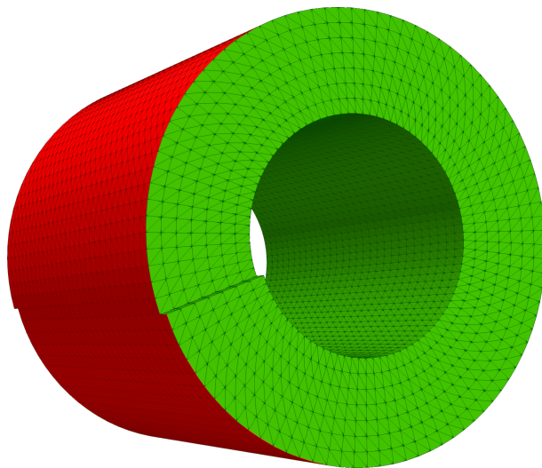
FIGURE 1: A short pipe mesh counting 20,000 vertices.
